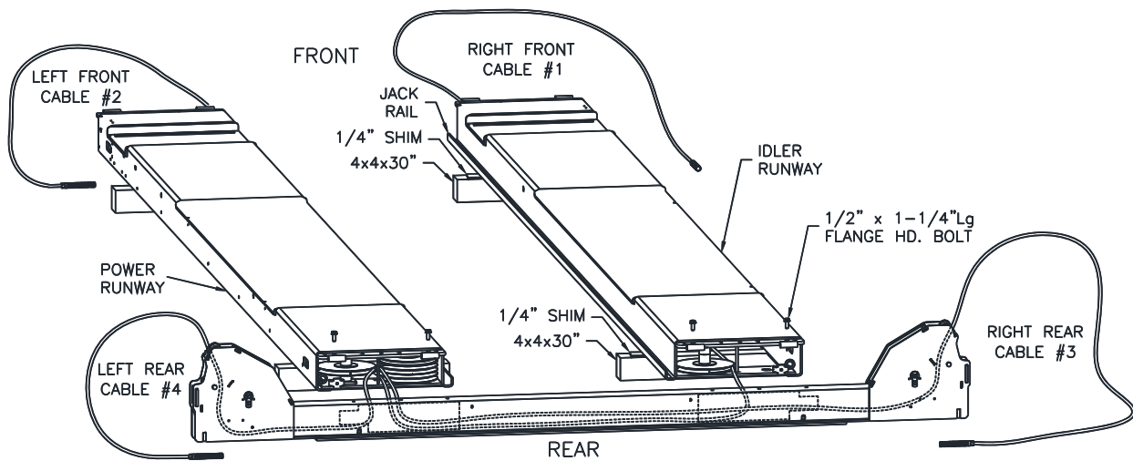
– Runway Layout
