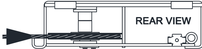
Fig 10 – Cable #1 Routing
