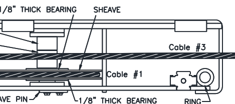
Fig 5 – Idler Runway Single-Stack
