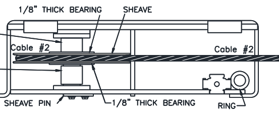
Fig 7 – Power Runway Single-Stack
