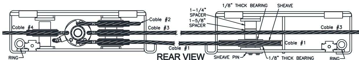
Fig 4 – Power Runway 3-Stack & Single Stack
