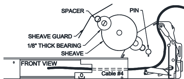
Fig 8 – Cable #4 Routing
